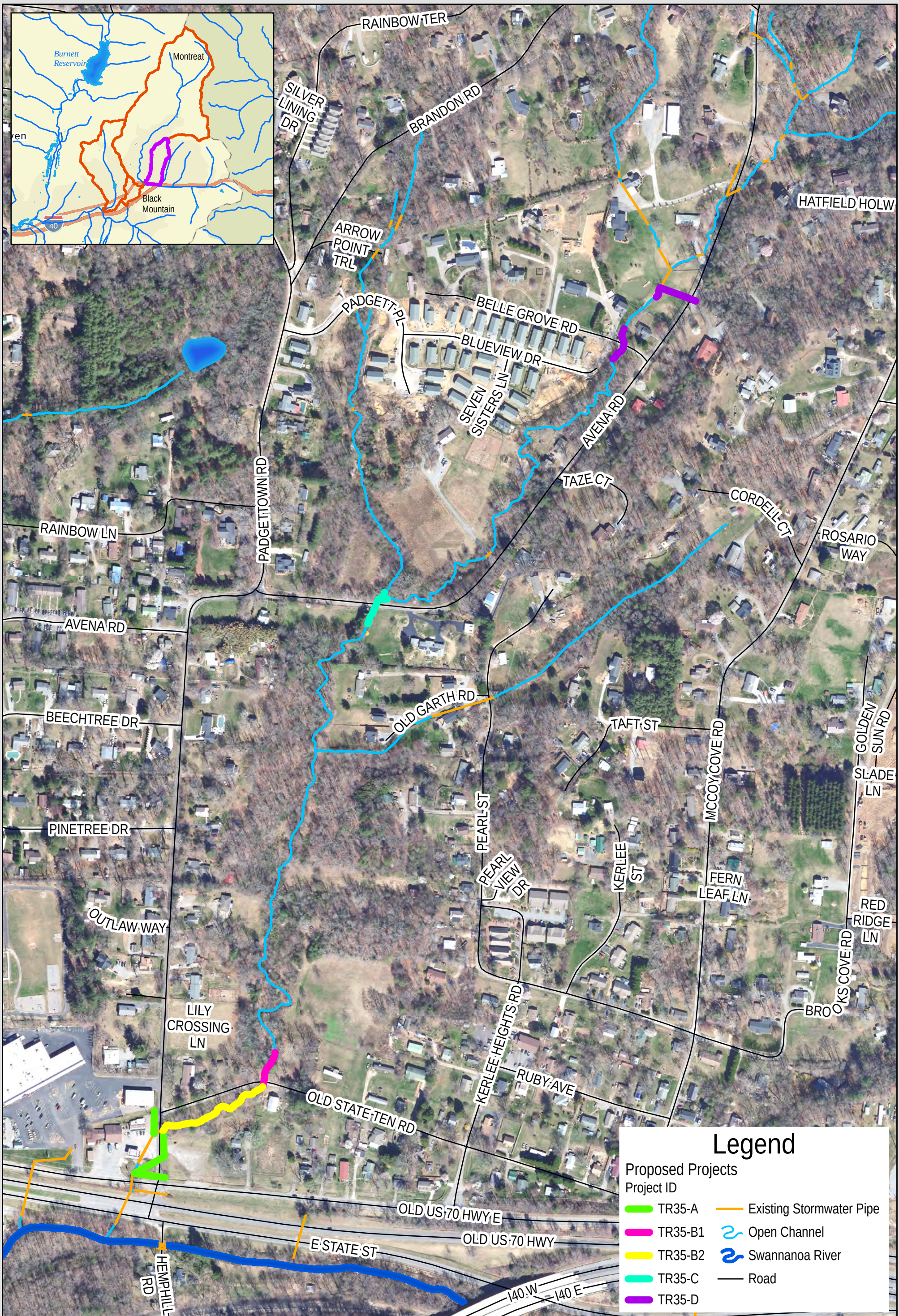
Figure ES-8: Proposed Stormwater Improvement Projects AVENA ROAD/TRIBUTARY 35 PRIMARY SYSTEM Town of Black Mountain Stormwater Master Plan
