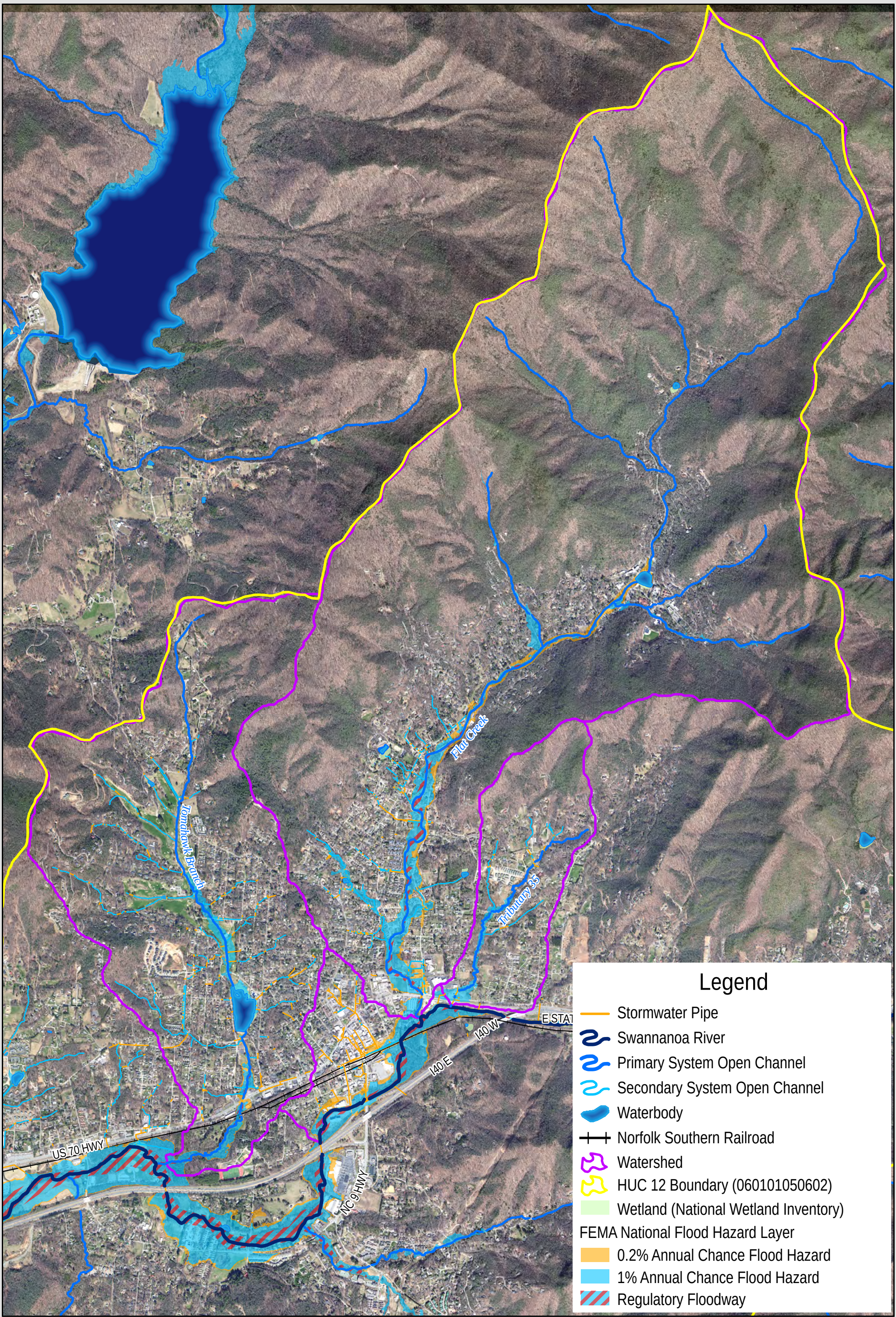
Figure 2-3: Hydrology TOWN OF BLACK MOUNTAIN, NC Town of Black Mountain Stormwater Master Plan
