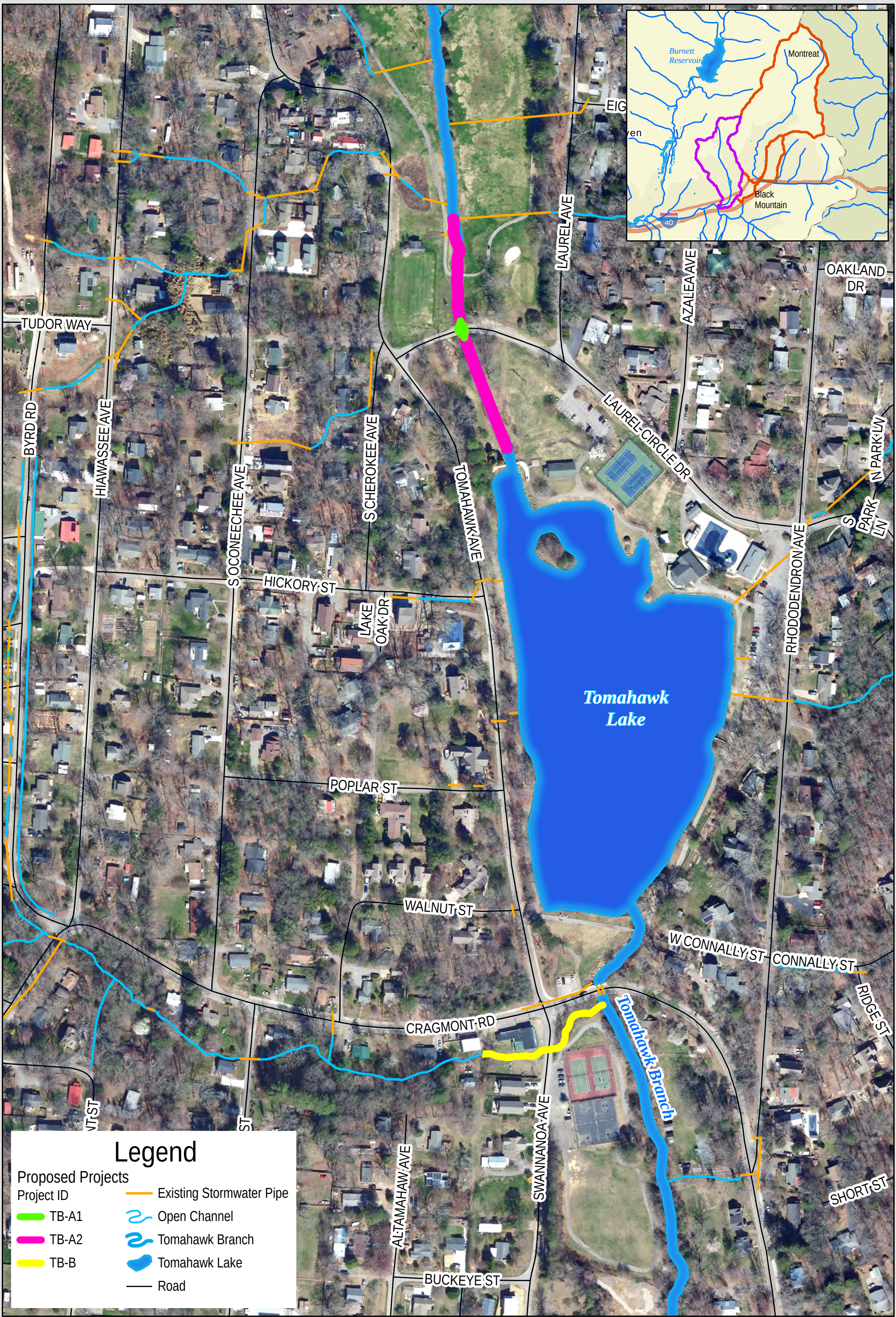
Figure ES-6: Proposed Stormwater Improvement Projects TOMAHAWK BRANCH PRIMARY SYSTEM Town of Black Mountain Stormwater Master Plan
