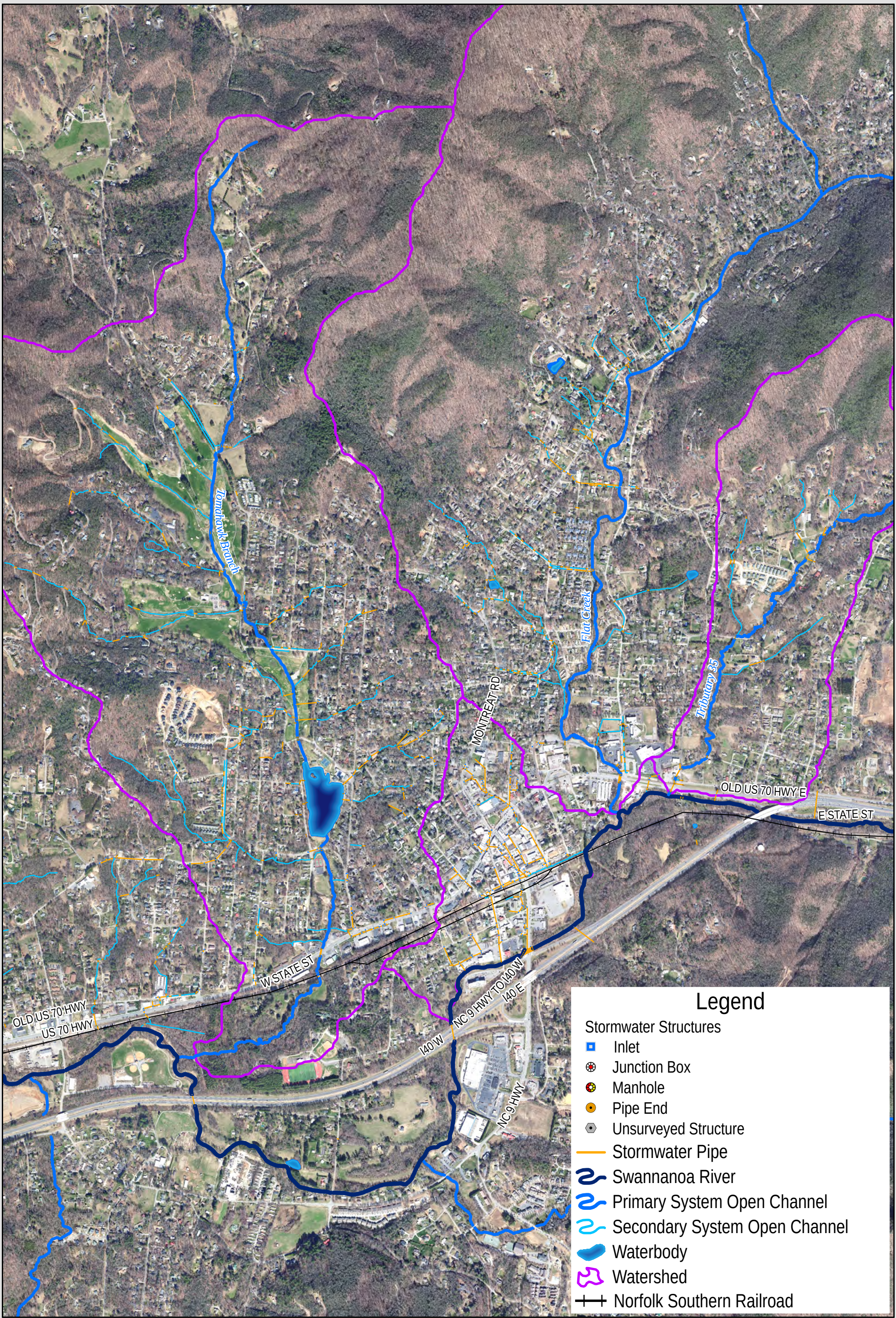
Figure 2-1: Stormwater Inventory TOWN OF BLACK MOUNTAIN, NC Town of Black Mountain Stormwater Master Plan
