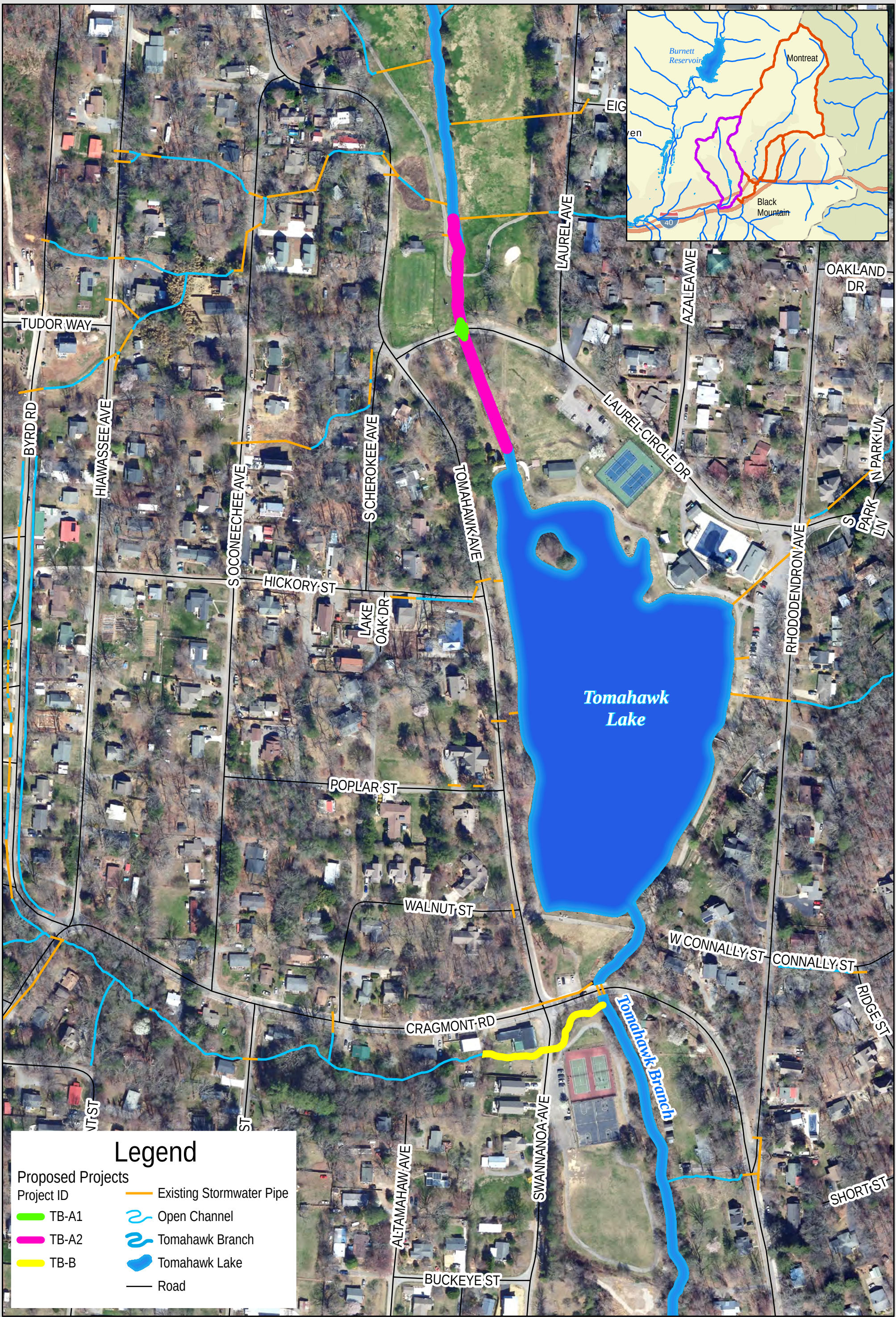
Figure 5-4: Proposed Stormwater Improvement Projects TOMAHAWK BRANCH PRIMARY SYSTEM Town of Black Mountain Stormwater Master Plan
