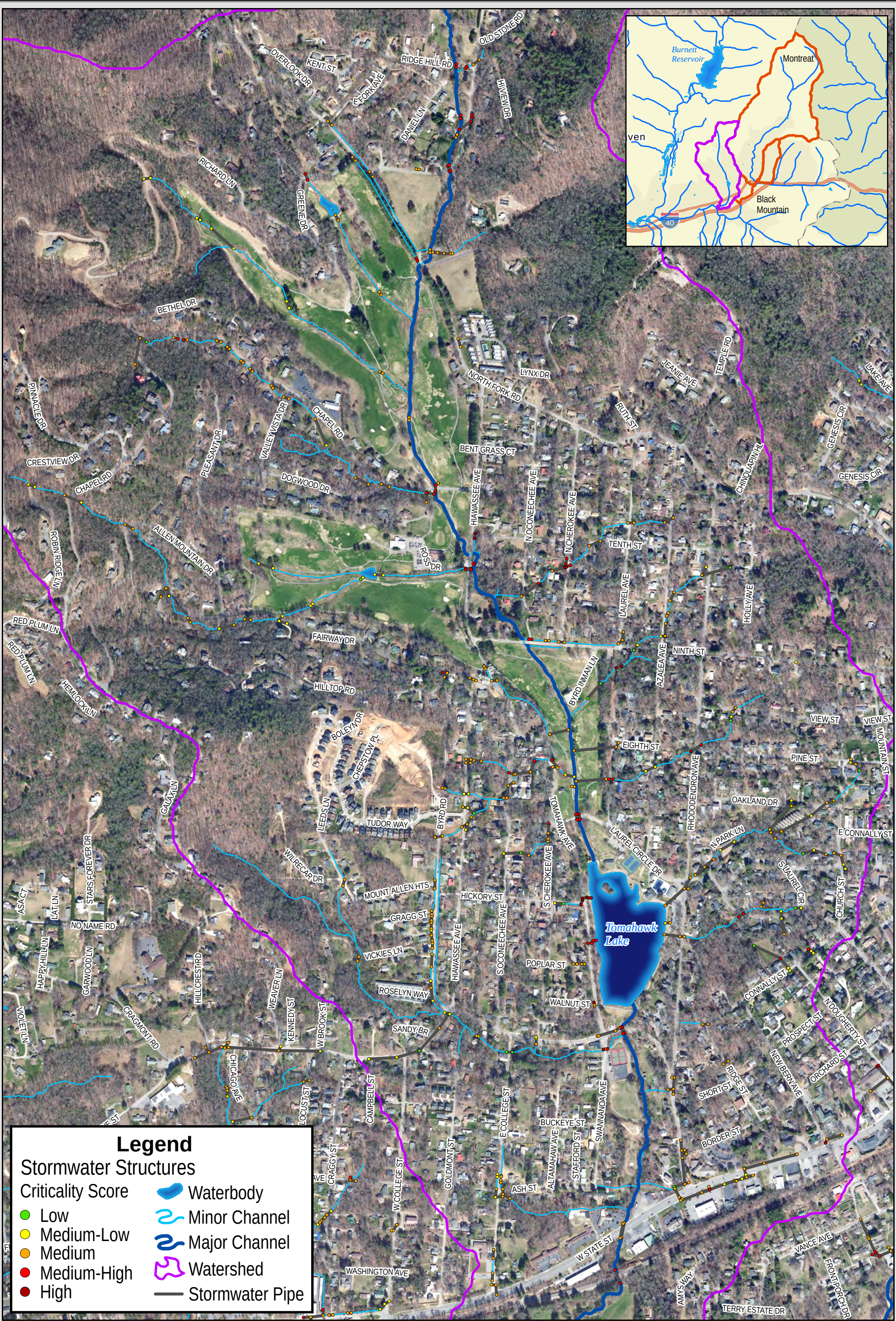
Figure D-2: Criticality Analysis Results - Stormwater Structures TOMAHAWK BRANCH PRIMARY SYSTEM Town of Black Mountain Stormwater Master Plan
