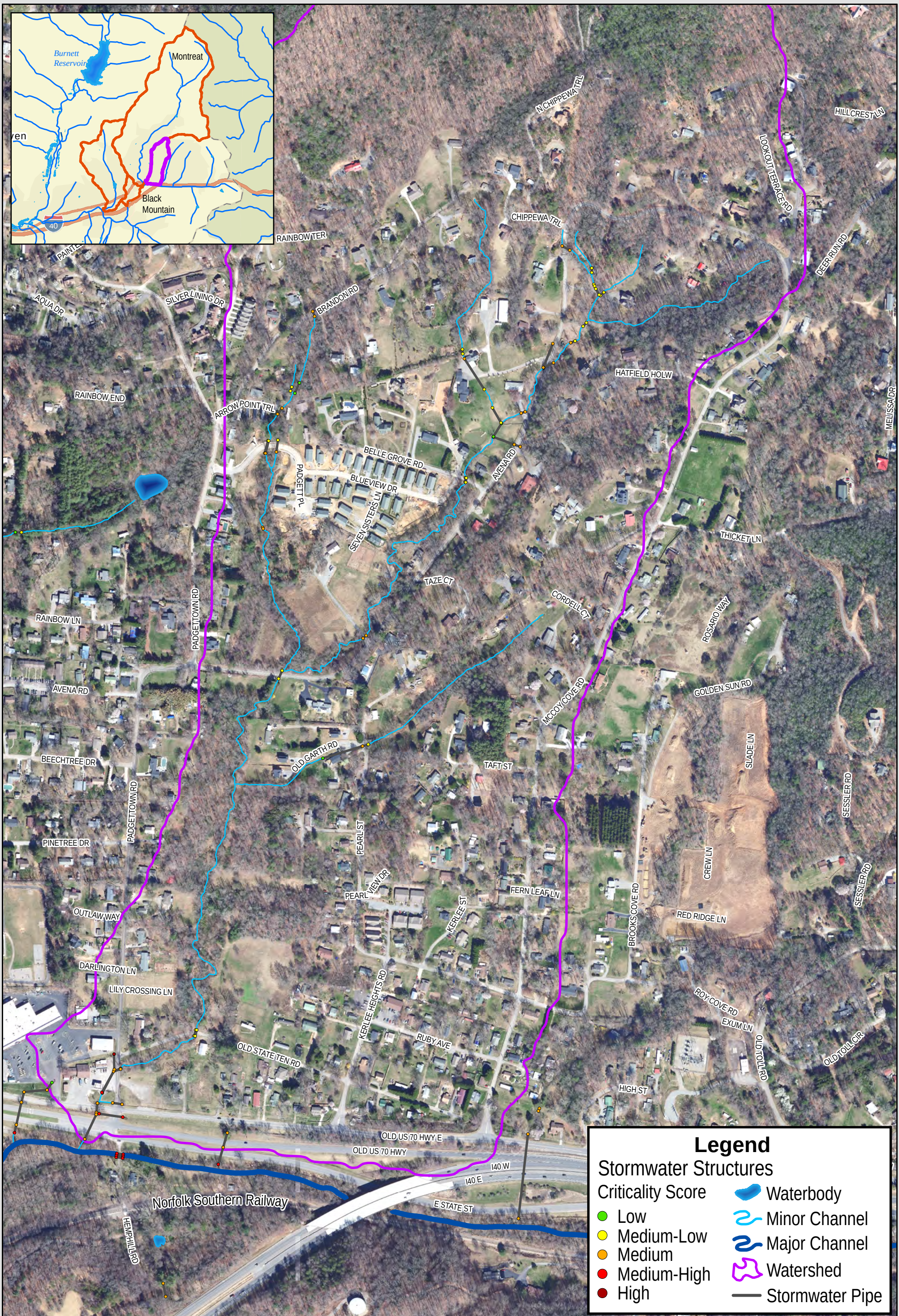
Figure D-4: Criticality Analysis Results - Stormwater Structures AVENA ROAD/TRIBUTARY 35 WATERSHED Town of Black Mountain Stormwater Master Plan
