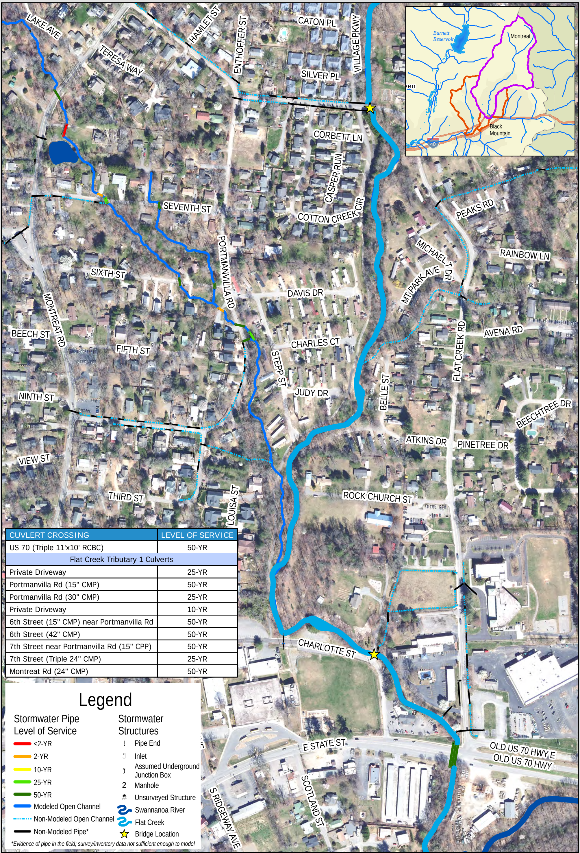
Figure 5-7: Proposed Conditions Level of Service FLAT CREEK TRIBUTARY 1 PRIMARY SYSTEM Town of Black Mountain Stormwater Master Plan
