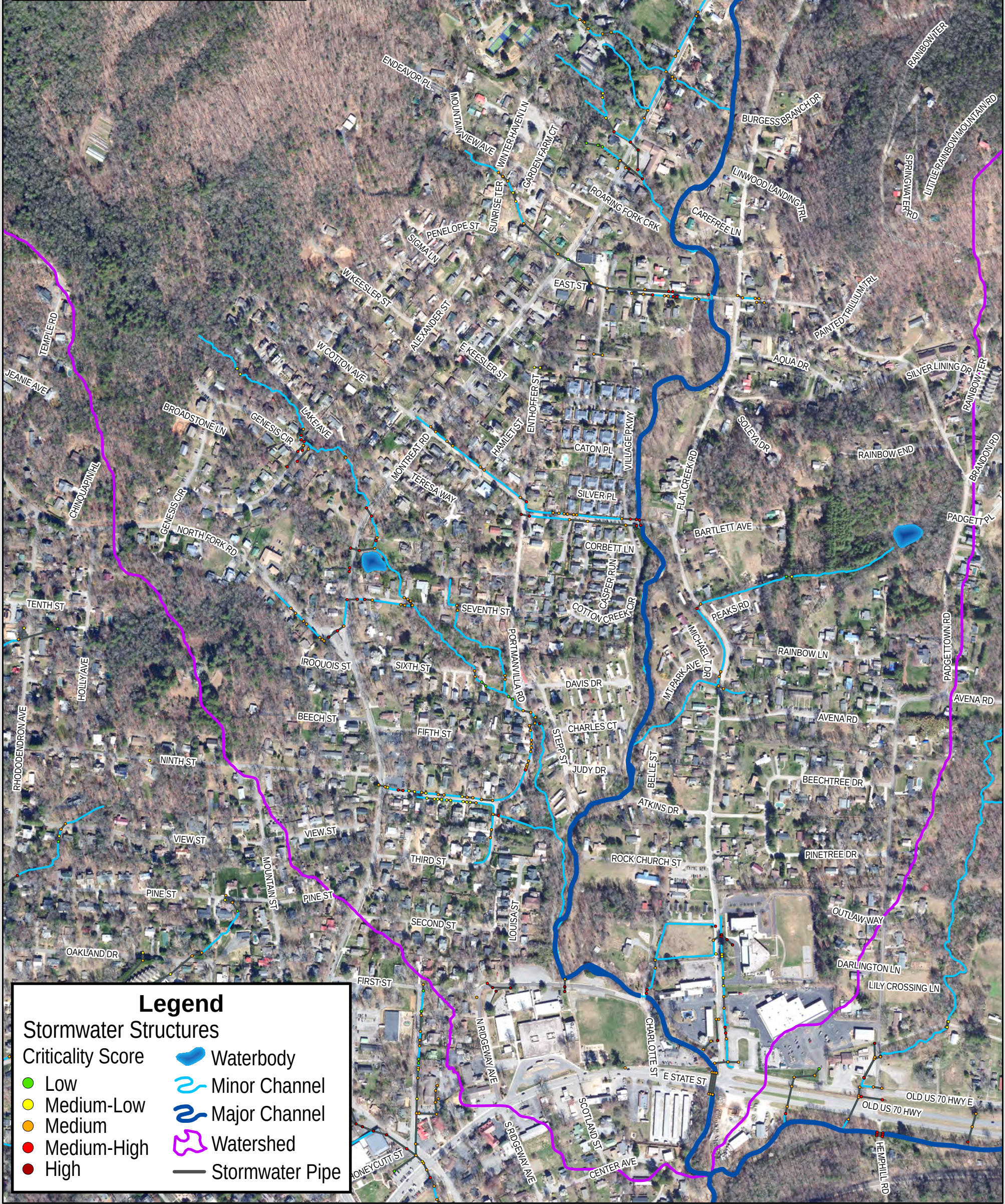
Figure D-3: Criticality Analysis Results - Stormwater Structures FLAT CREEK TRIBUTARY 1 PRIMARY SYSTEM Town of Black Mountain Stormwater Master Plan
