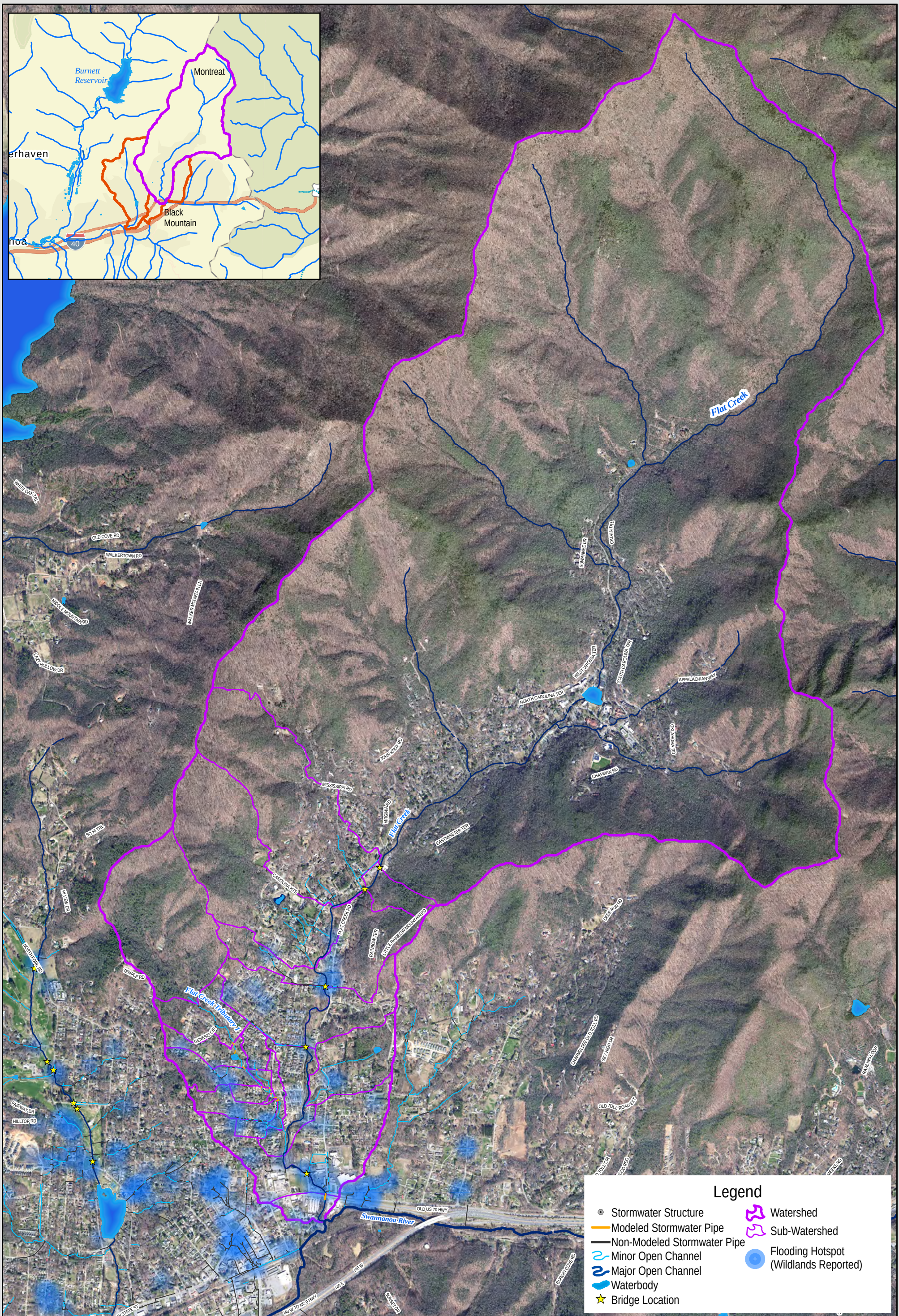
Figure 3-8: Flat Creek Tributary 1 Primary System Town of Black Mountain Stormwater Master Plan
