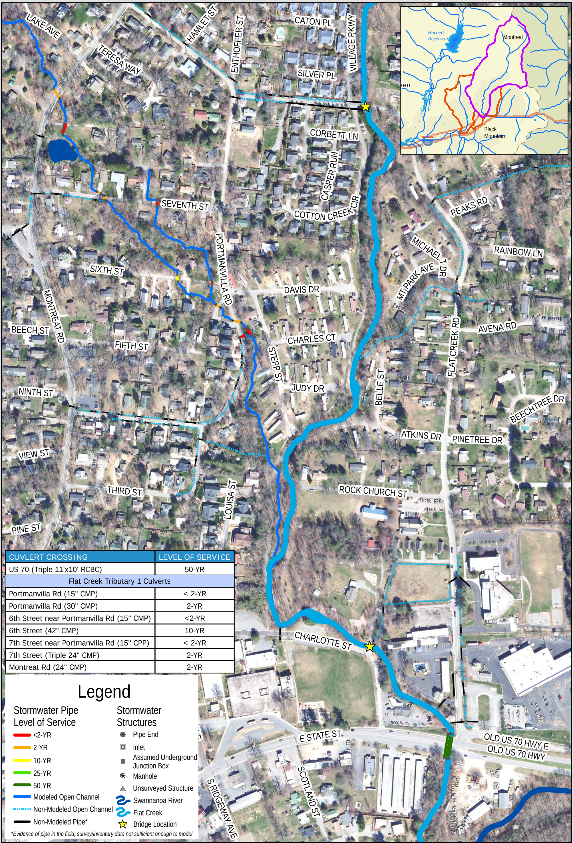
Figure 3-9: Existing Conditions Level of Service FLAT CREEK TRIBUTARY 1 PRIMARY SYSTEM Town of Black Mountain Stormwater Master Plan
